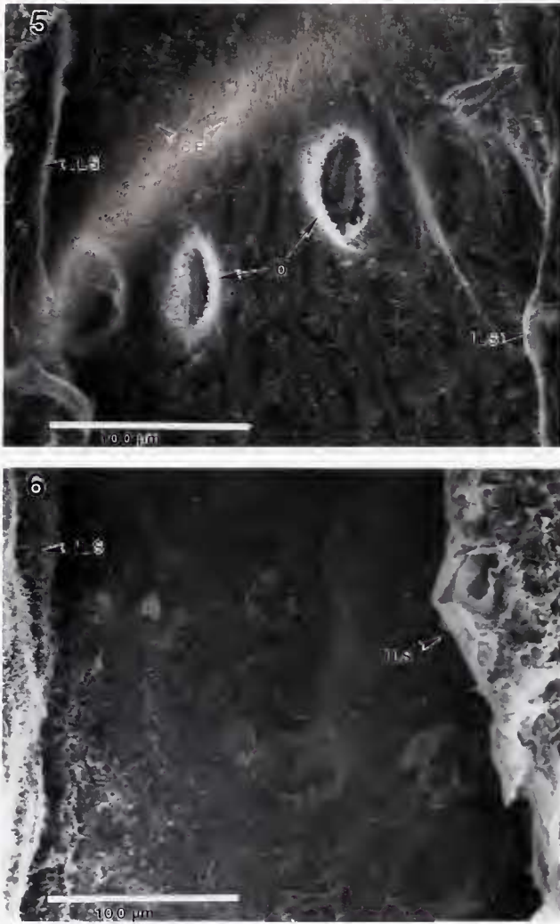
Figure 5. Scanning electron micrograph of the inner lamellar surface of a secondary water tube of a gravid marsupial gill of Anodonta cataracta . Water pumped through the interfilament canals by lateral cilia enters the secondary water tubes through well-defined ostia (O). Lamellar walls consisted primarily of ciliated epithelial cells (CE). The edges of the interlamellar septa (ILS) connecting the opposing lamellae and forming the anterior and posterior walls of the secondary water tube are also visible.
